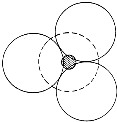
TETRAHEDRON 0.2248
