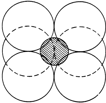
TRIGONAL PRISM 0.5276
