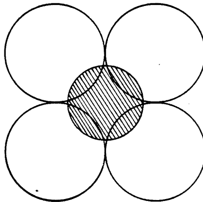
CUBE 0.7321
