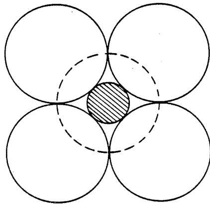
OCTAHEDRON 0.4142
