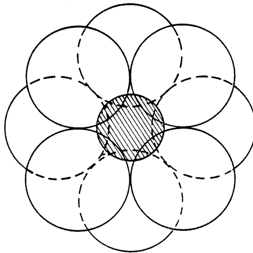
SQUARE ANTIPRISM 0.6454
